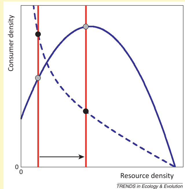
Figure 1. The consumer (red) and resource (blue) isoclines in the phase space of an unstructured consumer-resource model when resource dynamics follow logistic (unbroken line) or semi-chemostat dynamics (broken line). The dots represent the internal equilibria for logistic (grey) and semi-chemostat (black) resource dynamics when mortality is increased (arrow). Note that with logistic growth, the equilibria to the left of the maximum are unstable and the system exhibits limit cycles, which are not shown.
